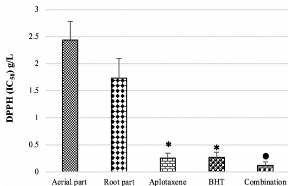
Figure 3. Antioxidant activity (IC 50 g/L) of essential oil of C. acaulis by DPPH method (*significant p≤0.01 compared to aerial and root parts; ●significant p≤0.01 compared to aplotaxene and BHT)
