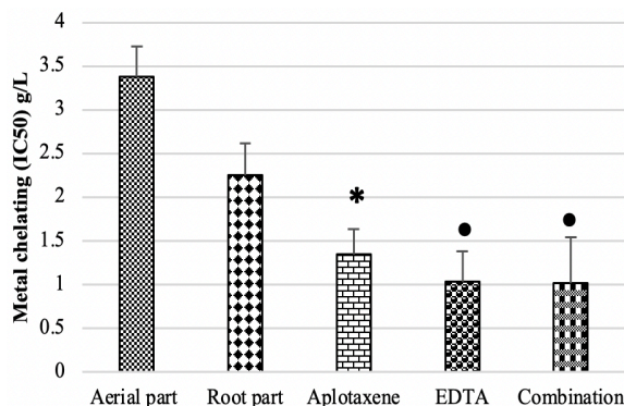
Figure 4. Antioxidant activity (IC 50 g/L) of essential oil of C. acaulis by Metal Chelating Method (*significant p≤0.01 compared to aerial and root parts; ●significant p≤0.01 compared to aplotaxene and EDTA).
