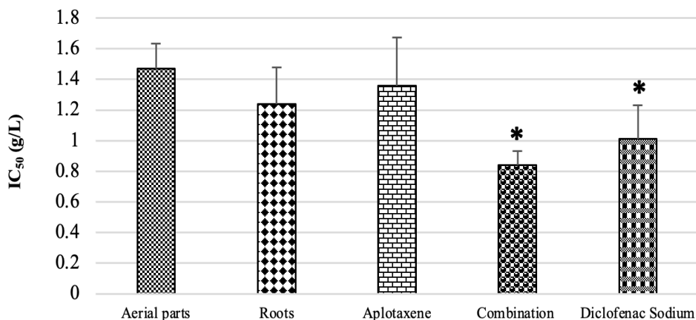
Figure 6. IC_{50} values of C. acaulis essential oils, aplotaxene, sodium diclofenac and their combination
